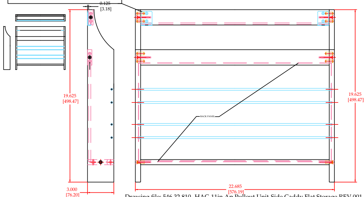
Drawing file: 546.32.810- HAC-11in.Ap Pullout Unit-Side Caddy Flat Storage.REV.001.dwg Material: Birch plywood and Birch/maple solids
